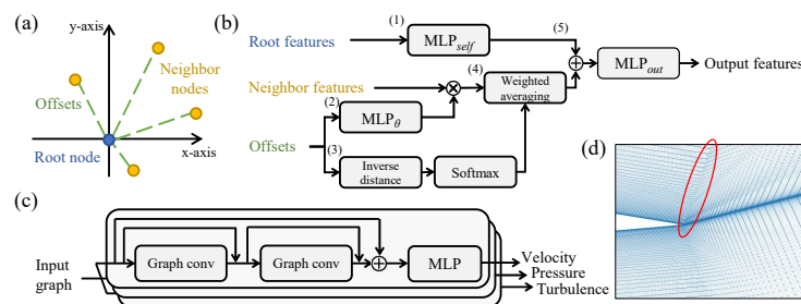
Figure 2: Offset-based graph convolution architecture. (a) Spatial relationships: root node (blue), neighbor nodes (orange), offset vectors (green dashed lines). (b) Convolution workflow: key steps including self-feature update, kernel weight generation, attention weights, aggregation, and feature fusion. (c) Our method uses three dedicated GNN models for different predictions. (d) Hybrid graph construction with kNN connections and abrupt connectivity transition.
