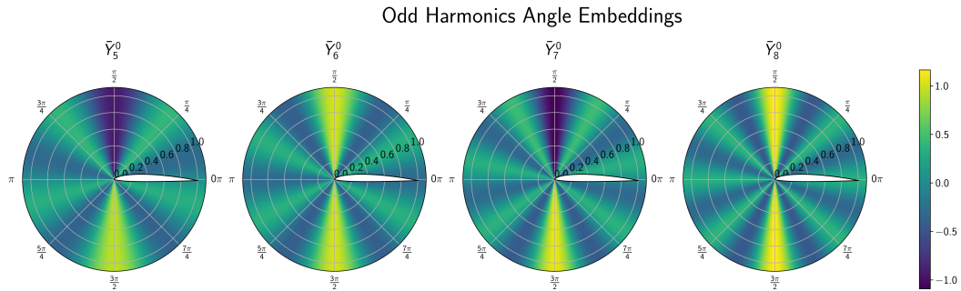
Figure 28: Odd harmonics embeddings of angles in the leading edge coordinate system with m = 0 and varying order \ell .
