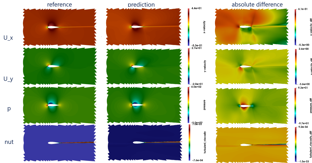
Figure 15: Illustration of the result on the first sample of the test set for the offset-based approach.
