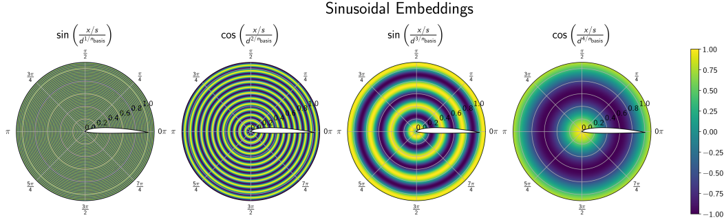
Figure 26: Sinusoidal embeddings of varying frequency for distance in the leading edge coordinate system.
