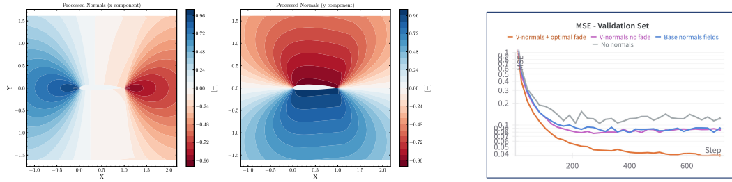
(a) Visualization of the volumetric normals field around an airfoil, showing the x-component (left) and y-component (right) with a smooth transition from the surface to the far field. (b) Validation loss comparison when volumetric normals are incorporated as input features.
