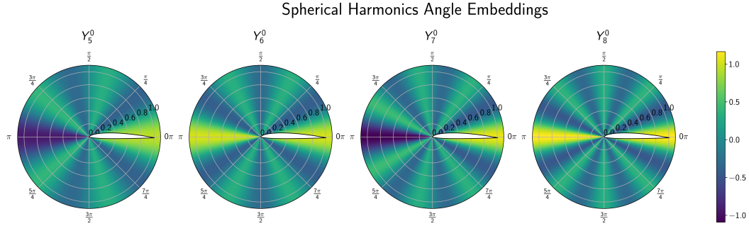
Figure 27: Spherical harmonics embeddings of angles in the leading edge coordinate system with m = 0 and varying order \ell .
