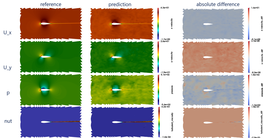
Figure 20: Illustration of the result on the first sample of the test set for the MARIO approach.
