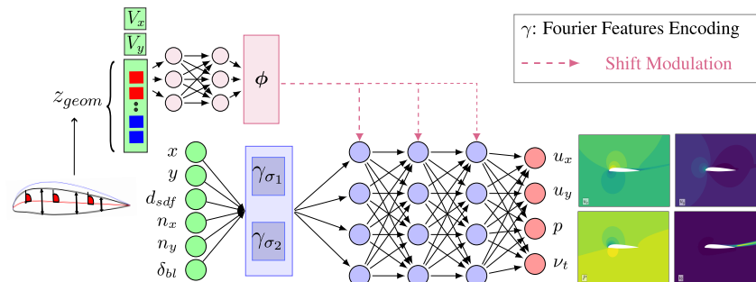
Figure 3: MARIO conditional neural field architecture. Input features (spatial coordinates, SDF, and engineered fields) are processed through multiscale Fourier feature encoding ( \gamma ). The hypernetwork processes the conditioning vector z (consisting of inflow conditions and geometric parameters) to generate layer-specific modulation vectors \phi . These modulations are applied to each intermediate layer of the main network via shift modulation.
