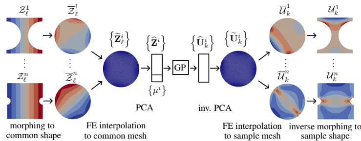
Figure 1: Illustration of MMGP inference workflow for the prediction of an output field [22].
