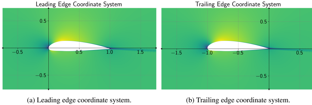
Figure 23: Leading and trailing edge coordinate systems. The leading and trailing edge coordinate systems enable the model to be able to distinguish between the three regimes of dynamics described in Figure 22.
