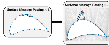
Figure 4: Illustration of surface-to-volume message passing in the GeoMPNN framework [30].
