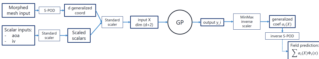
Figure 10: Workflow of the machine learning part of MMGP
