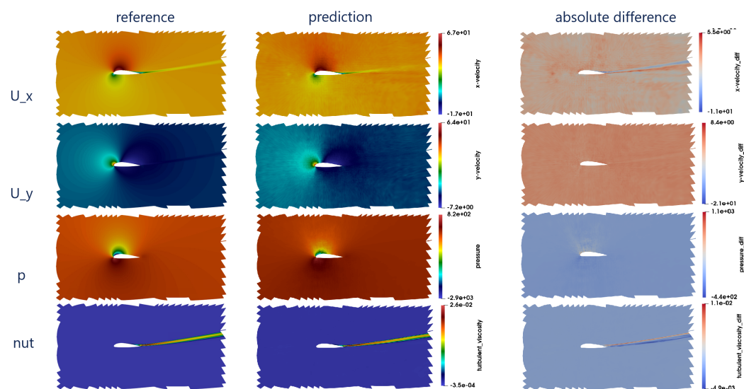
Figure 34: Illustration of the result on the first sample of the test_ood set for the GeoMPNN approach.
