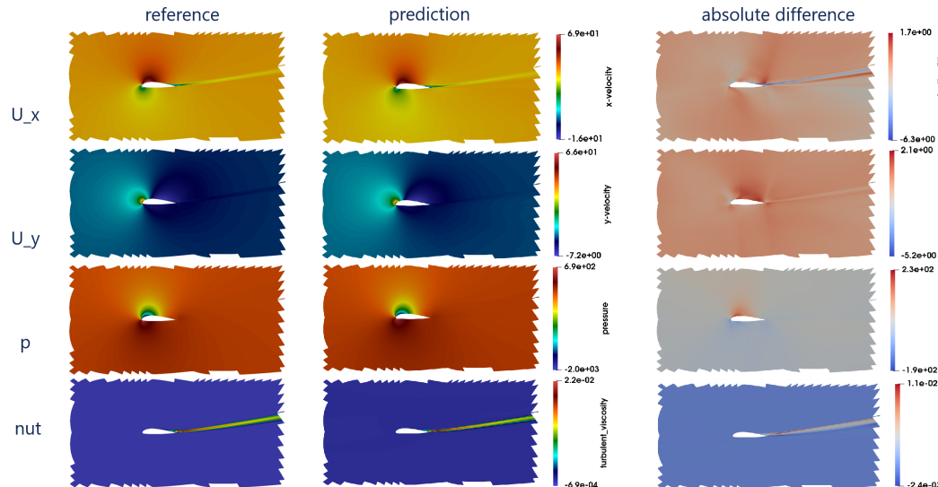
Figure 16: Illustration of the result on the first sample of the test_ood set for the offset-based approach.
