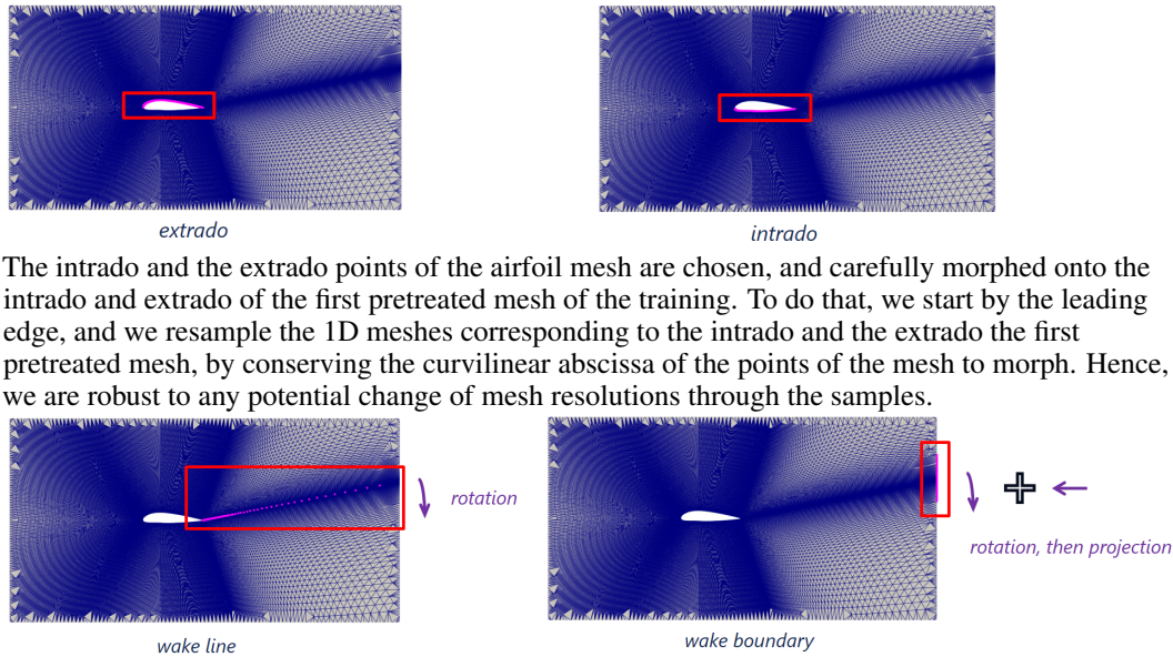
Figure 8: Transformation of the control points for the Radial Basis Function morphing. We identify the points at the center of the wake, except the one on the boundary, and apply a rotation to align them onto an horizontal line. Then, the right boundary condition must be transformed in a way that the points stay on the boundary box, but the element are stretched above the wake, and compressed below (in the configuration of the figure). The points close to the wake being extremely close, we prefer imposing the same rotation as the wake (and reprojecting them onto the boundary box), and we apply the stretching/compression to the other points of the boundary. The points of the top, bottom and left boundary are kept fixed.
