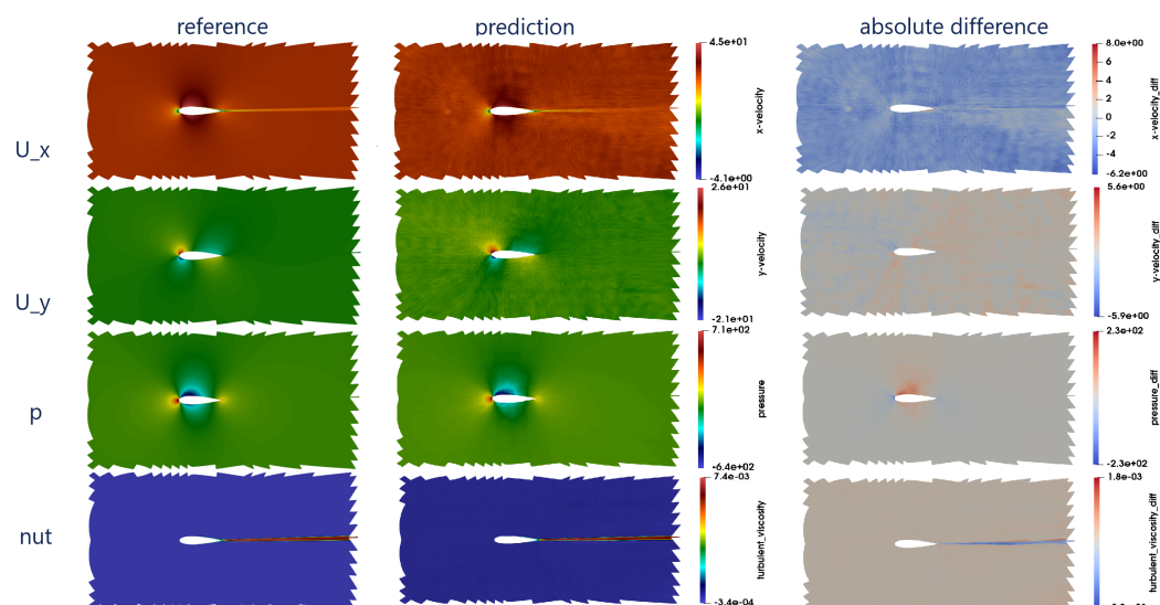
Figure 33: Illustration of the result on the first sample of the test set for the GeoMPNN approach.
