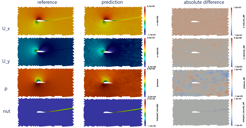
Figure 21: Illustration of the result on the first sample of the test_ood set for the MARIO approach.
