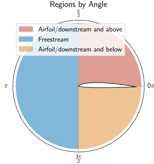
Figure 24: Regions by angle in the leading edge coordinate system. Polar angles can be used to derive both which of the regions along the x -axis defined in Figure 22 a mesh point is in, as well as where the point is vertically with respect to the airfoil. The same information is contained in the Cartesian form of the leading edge coordinate system, although the model must learn interactions between the x and y coordinates in order to derive it.
