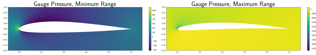
Figure 30: Pressure field with the least range ( left ) and with the greatest range ( right ).
