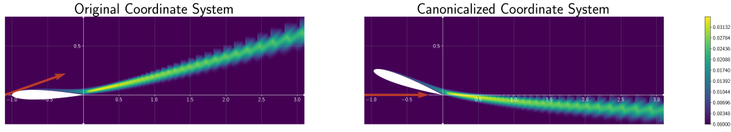
Figure 29: Turbulent viscosity and inlet velocity in the trailing edge coordinate system ( left ) and in the canonicalized trailing edge coordinate system ( right ). The direction of the inlet velocity, shown in red, is strongly associated with the direction of the non-zero parts of the turbulent viscosity field. After canonicalizing the coordinate system such that the inlet velocity is parallel with the x -axis, the non-zero parts of the turbulent viscosity are concentrated in the region around the x -axis for all examples.
