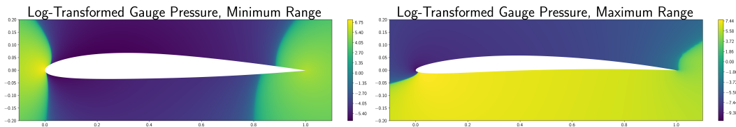
Figure 32: Log-transformed pressure field with the least range ( left ) and with the greatest range ( right ).
