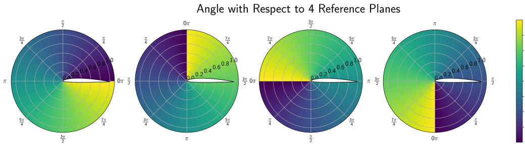
Figure 25: Angles in the leading edge coordinate system with respect to four different reference planes. Features in the POLAR model include angles with respect to all four reference planes.
