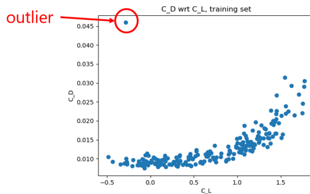
Figure 6: Outlier identifier in the training set by representing the drag coefficient with respect to the lift coefficient.
