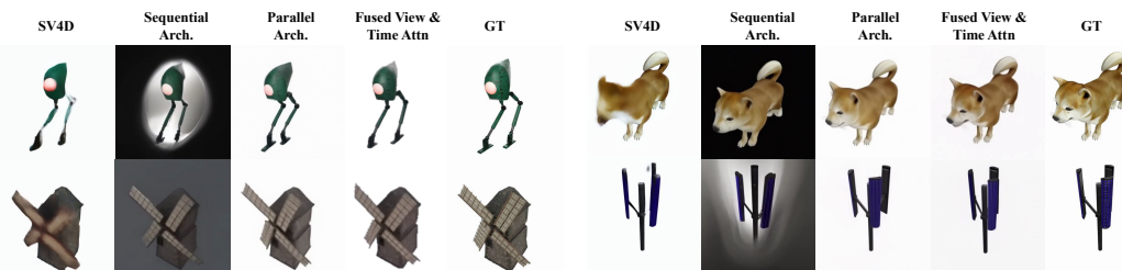
Figure S1: Qualitative comparison of the outputs of our proposed architecture (fused view-time attention) with our implementation of sequential and parallel architectures and SV4D [13].
