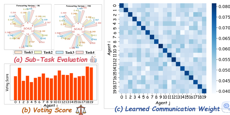
Figure 7: Case study of MAFS on ETTm2.
