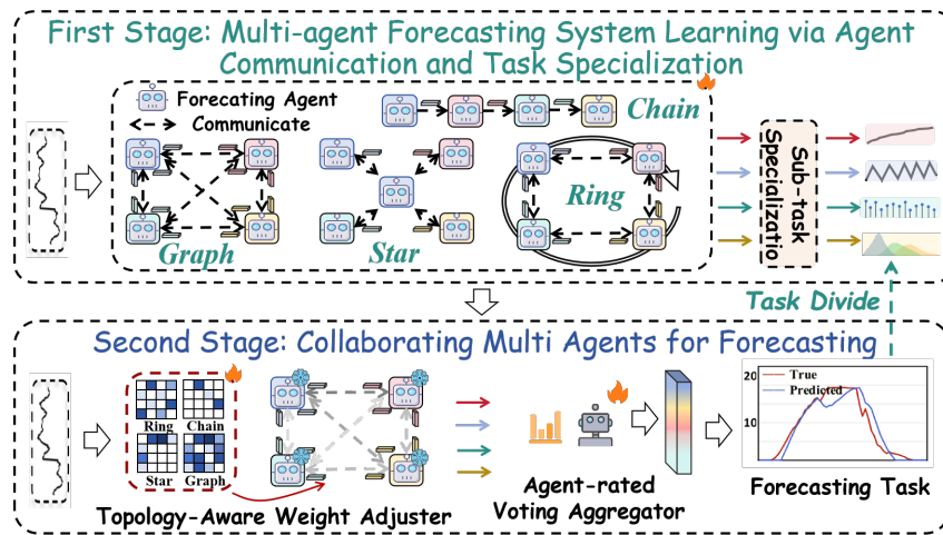
Figure 2: Overview of the two-stage learning in Multi-Agent Forecasting System.
