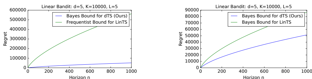
(a) Comparing our bound to the frequentist bound of LinTS in Abeille and Lazaric [2].
