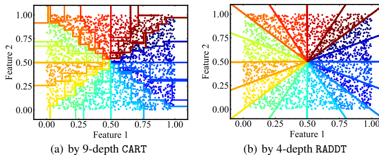
Figure 7: The decision boundary comparison for dataset “Syn-4”.
