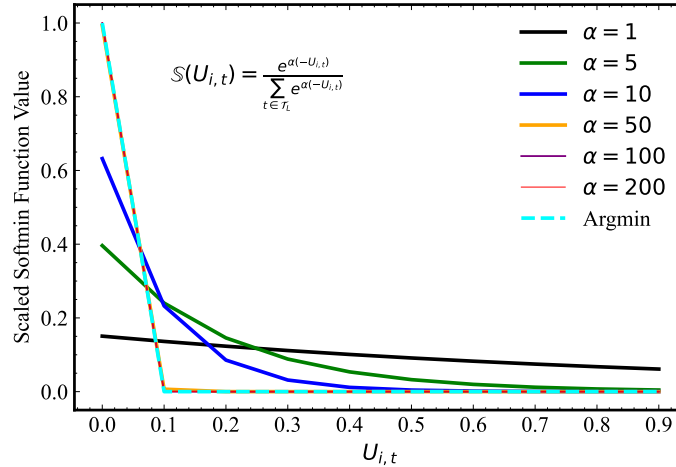
Figure 6: Comparison of scaled softmax function approximating Argmin behaviors under varying \alpha .
