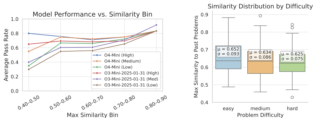
Figure 4: Left: Models with higher capacity (High) maintain relatively high performance even on low-similarity problems, while lower-capacity models benefit more from high-similarity problems. Right: Easy problems show slightly higher maximum similarity to past problems than hard ones, but the difference is limited.
