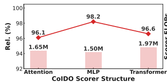
Figure 3: Ablations of different CoIDO Scorer architectures.
