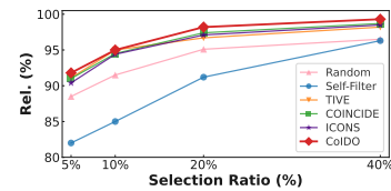
Figure 5: Performance vs. selection ratios \gamma .
