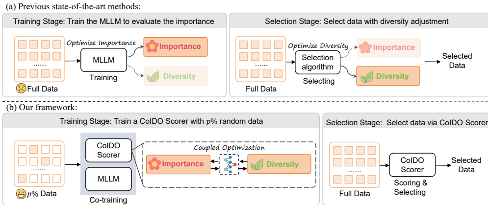
Figure 1: Previous state-of-the-art methods (e.g., TIVE [18] and ICONS [19]) treat importance and diversity as decoupled and independent components, using the entire data in the training stage. Our COIDO integrates importance and diversity in a coupled and reciprocal optimization, achieving superior data selection by utilizing only a fraction p\% ( p \ll 100 ) of the full dataset for model training and without any specialized algorithm in the selection stage.
