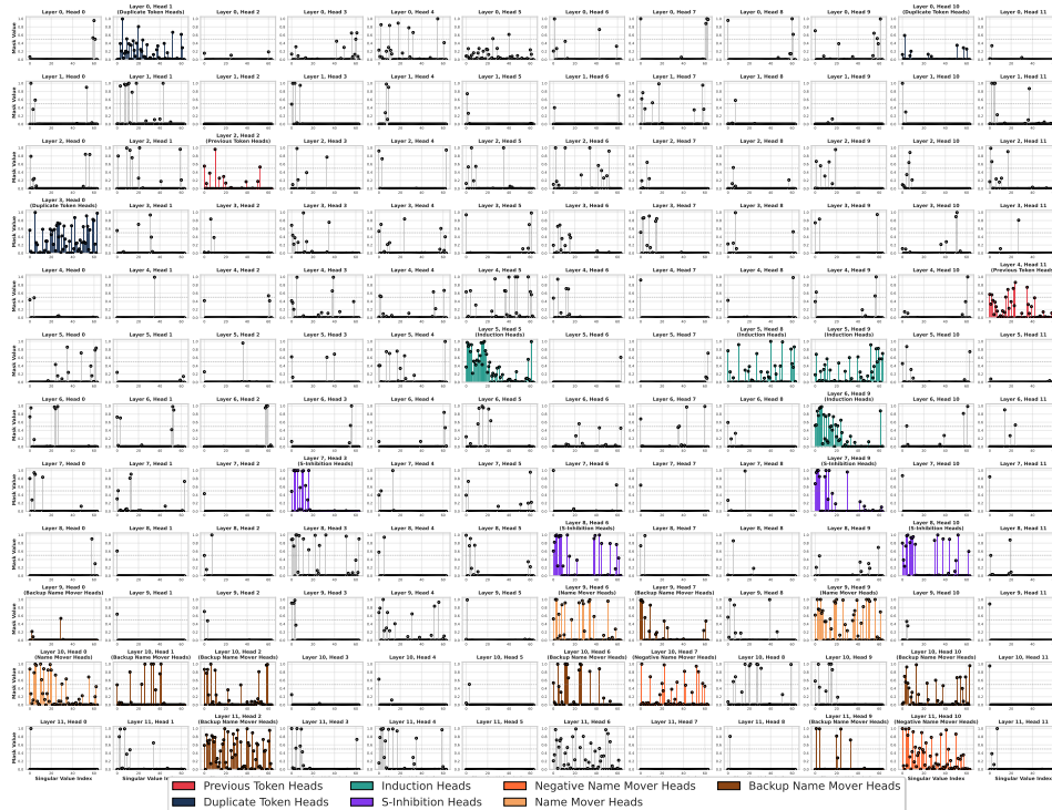
Figure 1: Learned singular value masks for Query-Key ( \mathbf{W}_{\text{aug}}^{\text{QK}} ) matrices across all attention heads in the model. High mask activations correspond to circuit components previously identified for the IOI task [Wang et al., 2022]. Each head exhibits sparsity along its singular directions, revealing the fine-grained subspaces driving task behavior.
