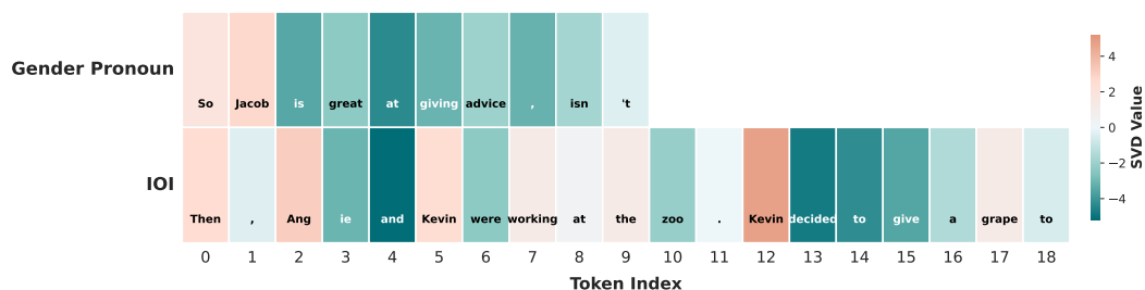
Figure 11: The figure above shows an instance of attention scores of the final token for component S_7 of head 9.6. It demonstrates that S_7 consistently act as an Entity action separator by giving the highest attention score to Name and object entities, and the least attention score to actions.
