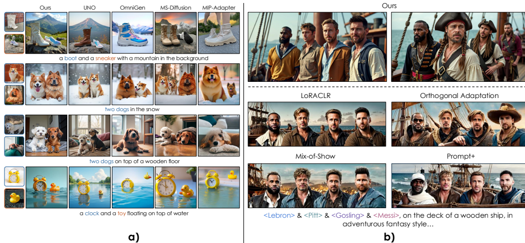
Figure 6: Multi-concept personalization across domains. (a) Non-human and object-centric composition: LoRASHop extends beyond identity personalization to animals, footwear, and objects, accurately preserving shape and texture semantics without retraining or external guidance. (b) Human multi-subject composition: LoRASHop disentangles and blends multiple identity LoRAs (e.g., <Lebron> , <Pitt> , <Messi> , <Gosling> ), maintaining subject fidelity and spatial coherence. Compared to baselines; LoRACLRL, Mix-of-Show, Prompt+, Orthogonal Adaptation, UNO, OmniGen, MS-Diffusion, and MIP-Adapter, LoRASHop preserves concept boundaries and contextual consistency while avoiding feature entanglement. Quantitative results for non-human concepts and occlusion-heavy overlapping cases are provided in the supplementary material.
