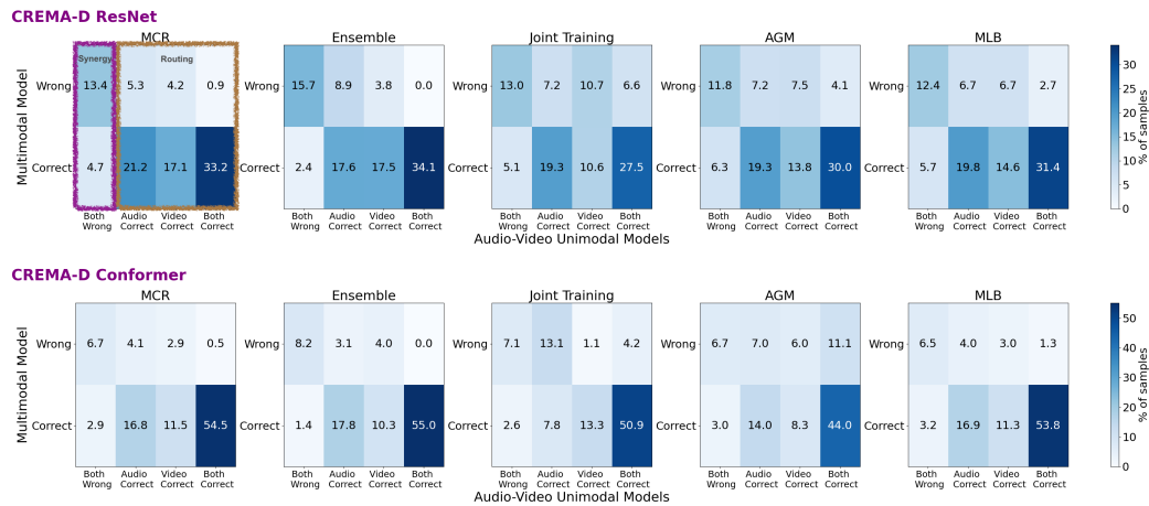
Figure 4: Error comparison on the CREMA-D dataset across unimodal and multimodal models (MCR, Ensemble, Joint Training, AGM, MLB). Each matrix summarizes model performance based on unimodal prediction correctness. MCR performs best when at least one unimodal branch is correct (brown box), effectively preserving modality-specific signals. However, AGM and MLB outperform MCR when both unimodal predictions fail, in the "Both Wrong" (purple box), indicating stronger synergy in those edge cases. Trends across other datasets are shown in Appendix A.11, with MOSI being a notable exception where MCR also excels in synergy.
