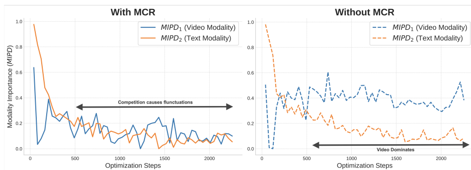
Figure 7: The plots show the two MIPD losses ( MIPD_1 and MIPD_2 ) for each modality, with (left) and without (right) regularization. With regularization, the losses exhibit an alternating pattern, demonstrating MCR's ability to dynamically explore multiple modality contribution combinations and prevent collapse into a single modality. Without regularization, the text modality initially contributes more strongly, but the video modality eventually outperforms and dominates.
