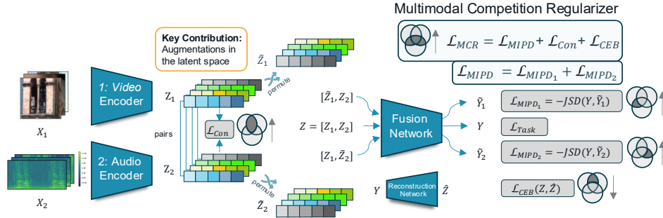
Figure 2: Multimodal Competition Regularizer (MCR): The diagram illustrates the MCR framework, which mitigates modality competition in multimodal learning. Raw data ( X_1 and X_2 ) are encoded into latent representations ( Z_1 and Z_2 ), which are then permuted to create \tilde{Z}_1 and \tilde{Z}_2 and the paired combinations. These combinations are passed through the Fusion Network to produce predicted outputs ( Y , \tilde{Y}_1 , \tilde{Y}_2 ). The comparison between predictions reveals each modality's contribution. For example, if Y \approx \tilde{Y}_1 , it shows that X_1 has little impact, and the model relies on X_2 . The MCR loss includes three components: \mathcal{L}_{MIPD} maximize the Jensen-Shannon divergence (JSD) between task output and permuted modality predictions. \mathcal{L}_{Con} aligns modality representations, while \mathcal{L}_{CEB} penalizes task-irrelevant information by reconstructing back to the latent space.
