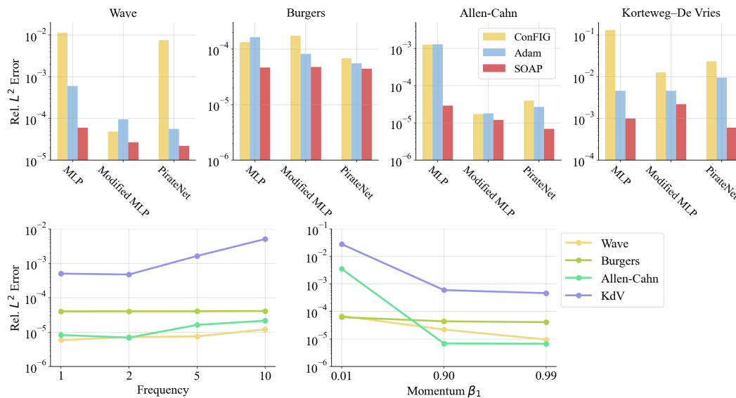
Figure 4: Optimizer performance comparison and ablation studies. Top: Relative L^2 error across PDE benchmarks using different optimizers. Bottom left: Relative L^2 error for varying preconditioner update frequencies in SOAP optimizer. Bottom right: Relative L^2 error with different momentum values in SOAP optimizer.
