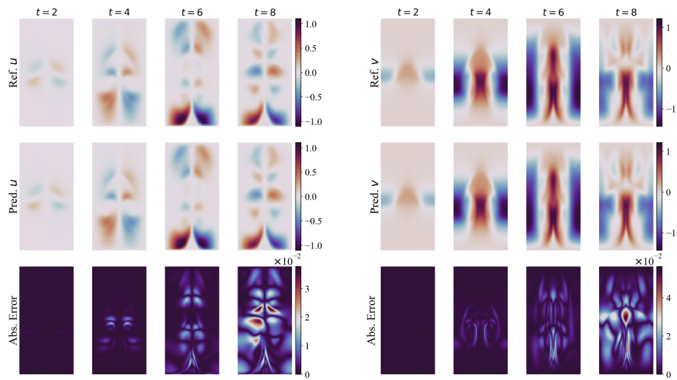
Figure 21: Rayleigh-Taylor instability . Comparison between reference solution and model predictions.
