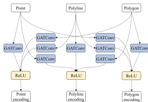
Figure 4: Detailed structure of the OSM encoder.
