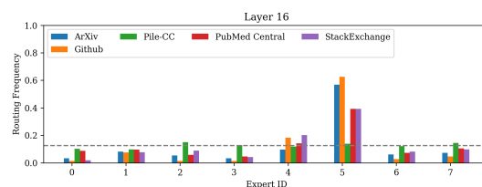
Figure 22: Domain Specialization for 8c1 DefaultMoE at Layer 16.
