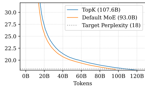
Figure 12: Default MoE beats a tuned TopK baseline on FineWeb. Our method reaches the target perplexity of 18 about 15% faster than the baseline TopK method, without introducing any additional overhead.
