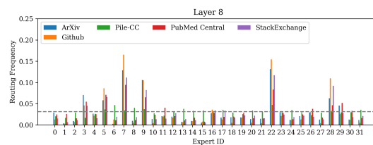
Figure 24: Domain Specialization for 32c4 DefaultMoE at Layer 8.
