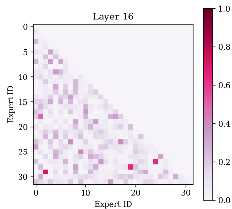
Figure 31: Expert Coactivation for 32c4 DefaultMoE at Layer 16.
