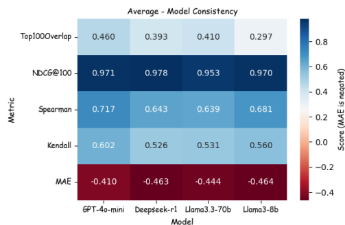
Figure 7: Consistency Heatmap
