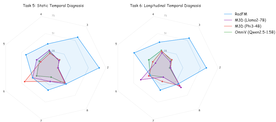
Figure 27: Zero-Shot Result of Task 5-6
