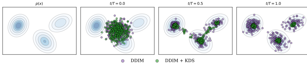
Figure 2: Kernel Density Steering (KDS) sharpens sample distributions in a 2D Mixture of Gaussians (MoG) toy problem. The target distribution p(x_0) consists of three distinct Gaussian modes. Samples are drawn using DDIM with the exact score function (purple dots) versus DDIM augmented with KDS (green dots, N = 50 particles). KDS guides particles through the reverse diffusion progresses, leading to significantly higher sample concentration at the mode peaks compared to standard DDIM.
