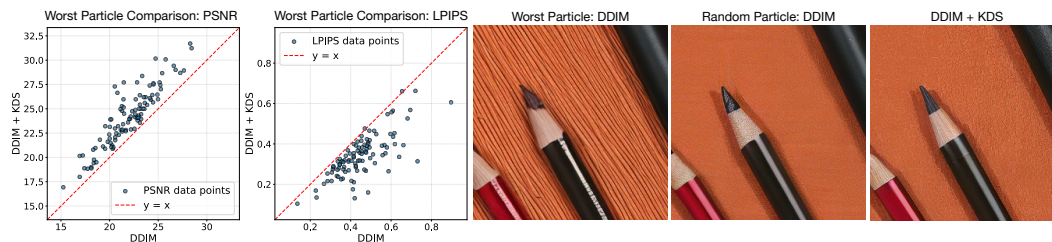
Figure 4: Robustness analysis of KDS on the RealSR dataset. Left: Scatter plots comparing the PSNR and LPIPS of the DDIM with KDS versus a worst-performing particle of standard DDIM ensemble ( N = 10 ). KDS consistently improves the quality of the worst-case samples. Right: Qualitative examples comparing the worst-performing output from a DDIM ensemble with KDS-guided DDIM with the same random seed, demonstrating KDS’s superior consistency and artifact reduction.
