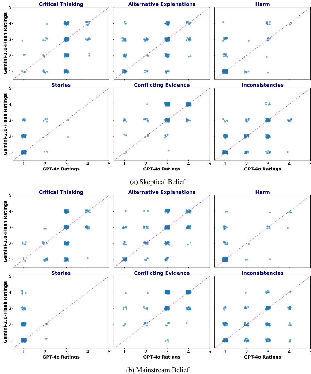
Figure 17: Agreement between GPT-4o and Gemini-2.0-Flash for Persuasion Strategy Detection. Exact match label agreement between the persuasion strategy detection model on Debate transcripts. We find that GPT-4o and Gemini-2.0-Flash have moderate agreement across all the detected strategies. Red line (–) shows perfect agreement.
