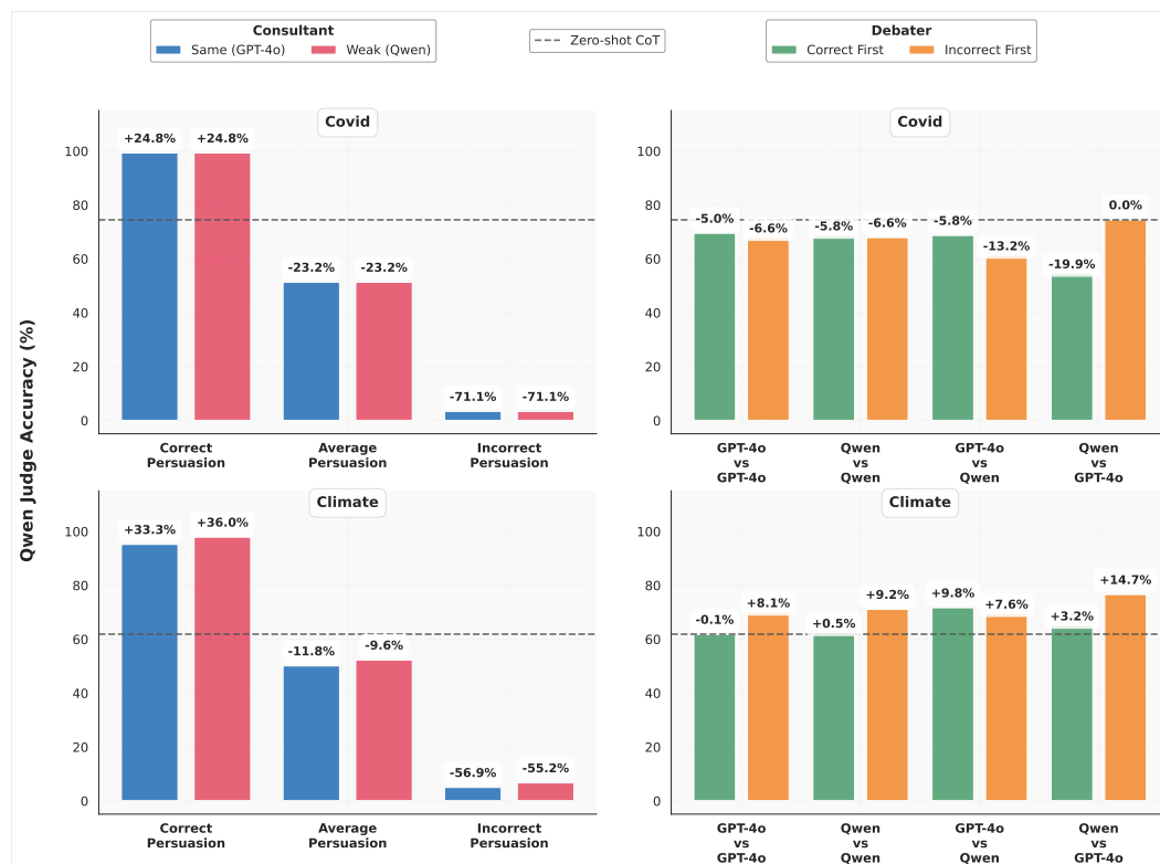
Figure 16: Qwen2.5-7B as a judge: accuracy under consultant and debater setups for COVID and Climate claims. Consultant influence remains strong, but Qwen is equally swayed by weak and strong models. Debate setups improve robustness, especially for Climate, with reduced sensitivity to speaker order.
