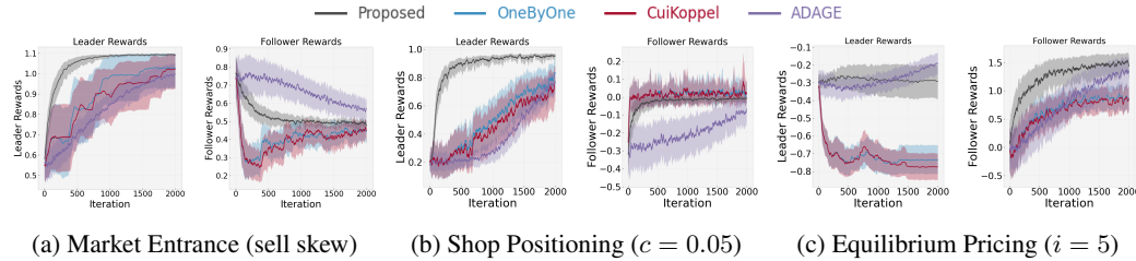
Figure 2: Convergence across environments, demonstrating bootstrapped mean and 5% confidence interval across 30 runs for the leader reward (left) and follower rewards (right).
