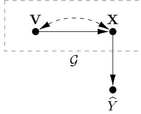
Figure 9: Diagrams used in the proof of Prop. 1.
