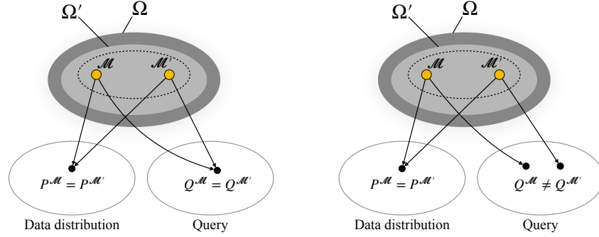
Figure 3: (Left) \Omega' is causally interpretable if a query can be uniquely computed from the observational data. (Right) A query cannot be uniquely computed from the observational data if \Omega' is not causally interpretable.
