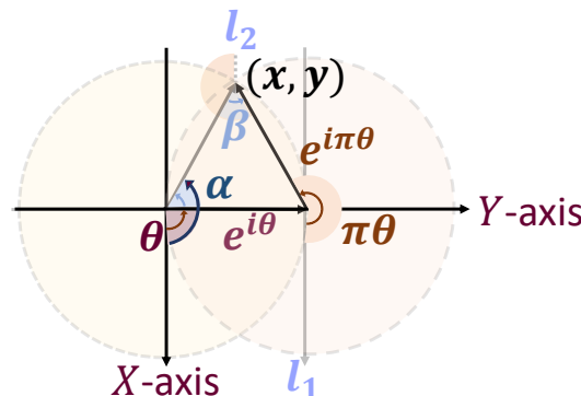
Figure 6: Geometric relationship in x + iy = e^{i\theta} + e^{i\pi\theta}
