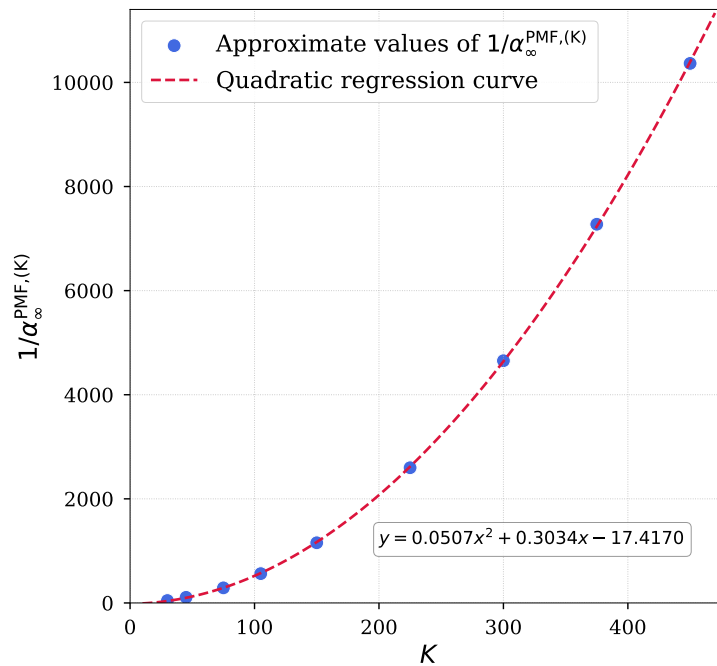
Figure 5. The approximate values of maximum step sizes 1/\alpha_{\infty}^{\text{PMF},(K)} under varying K . Here we take the average of the upper and lower bounds of \alpha_{\infty}^{\text{PMF},(K)} provided in Table 3 as an approximation of \alpha_{\infty}^{\text{PMF},(K)} and perform quadratic regression of 1/\alpha_{\infty}^{\text{PMF},(K)} on K . This fit achieves a mean squared error of 425.85 and R^2 of 0.99996, which indicates that 1/\alpha_{\infty}^{\text{PMF},(K)} indeed grows quadratically with respect to K , aligning with our theoretical results (Lemma E.3).
