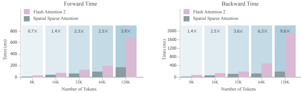
Figure 5: Comparison of the forward and backward time of our SSA and FlashAttention-2.
