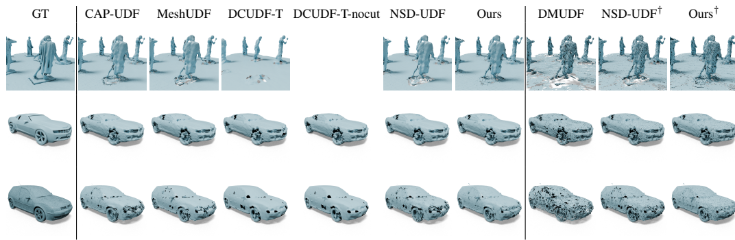
Figure 4: Qualitative comparison with existing methods (reconstruction from point clouds). Surface meshing results of neural UDFs at resolution of 512. Top: CAP-L 3D scenes. Middle: CAP-L car. Bottom: DiffUDF cars. † indicates that the method is combined with DMUDF.
