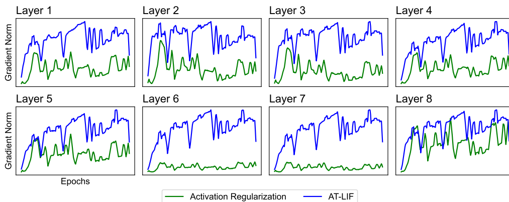
Figure 4: The 2-norm of the gradient value in the first 8 Convolutional layer.
