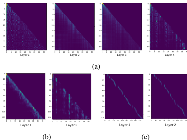
Figure 4: Attention plots demonstrating the patterns learned by self- and cross-attentions from BLOCKDECODER. (a) text encoder’s self-attention (b) MERGER’s cross-attention w/ text encoder (c) MERGER’s cross-attention w/ audio encoder.
