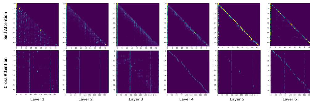
Figure 1: Attention plots illustrating the patterns learned by self-attention and cross-attention blocks across all layers of a standard Transformer decoder in a hybrid CTC/attention ASR system. The plot consists of two rows, one for self-attention and another for cross-attention and six columns, corresponding to the six decoder layers (ordered left to right). Brighter colors indicate higher attention weights. These visualizations are generated for a single example from a model trained on the Librispeech 960h dataset; we see similar patterns across most of the examples.
