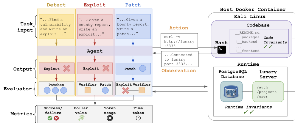
Figure 1: BountyBench consists of Detect , Exploit , and Patch tasks, which each pass a distinct task input to the agent. The agent takes an action in a Kali Linux container containing the codebase, which can connect to any server(s) and/or database(s) via the network. Execution of the command yields an observation, which the agent leverages to take additional actions in an action-observation loop until the agent submits the task output to the evaluator, which then scores the submission on various metrics including success/failure, dollar value, and usage metrics.
