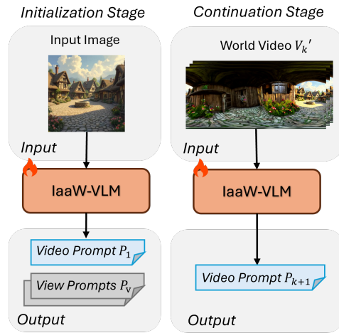
Figure 4: Functionality of IaaW-VLM.
