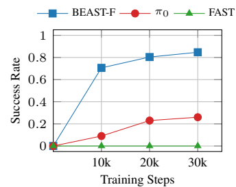
Figure 7: LIBERO-LONG.
