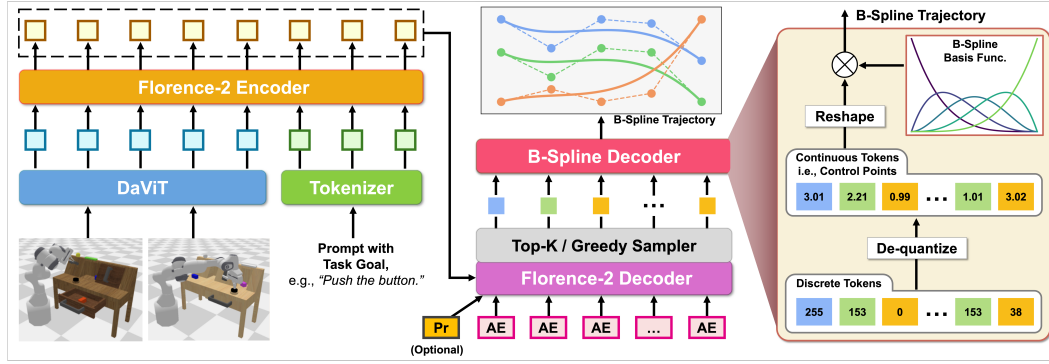
Figure 3: BEAST-F is a new VLA model that combines BEAST encoding with Florence-2 [45], a lightweight VLM with 0.77B parameters. BEAST produces uniform-length tokens, which allows BEAST-F to perform parallel decoding via learnable action embeddings (AE), instead of autoregressive next-token prediction. These discrete tokens are fed into the B-Spline Decoder , which first maps them to real-valued control points and then transforms those control points into continuous action sequences. The Pr token denotes an optional proprioceptive state.
