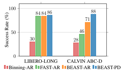
Figure 8: Tokenizer Comparison.
