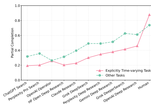
Figure 4: Average Partial Completion on explicitly time-varying tasks compared to other tasks.
